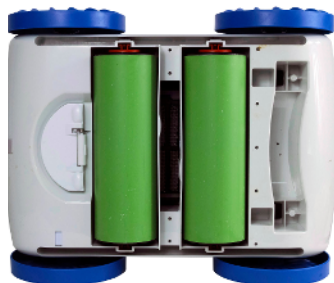
8.1: Manually rotate the green rollers. They should turn easily. If debris is blocking the rotation, remove the debris
